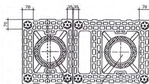
ZMS 42R+ ZMS 42LR+ ERLUS Ek - Rohr
